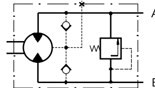
MMD Series with Integrated Internal Crossover Relief Valves A ↔ B, Δp = 100 bar (50 bar)
