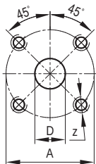
C GERMAN FLANGE
