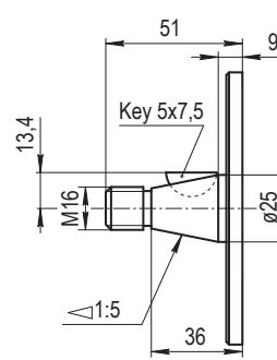
F4 GERMAN TAPERED 1:5
