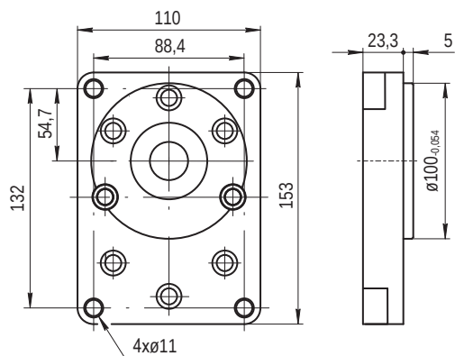
89 GERMAN \varnothing 100
