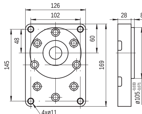
88 GERMAN \varnothing 105
