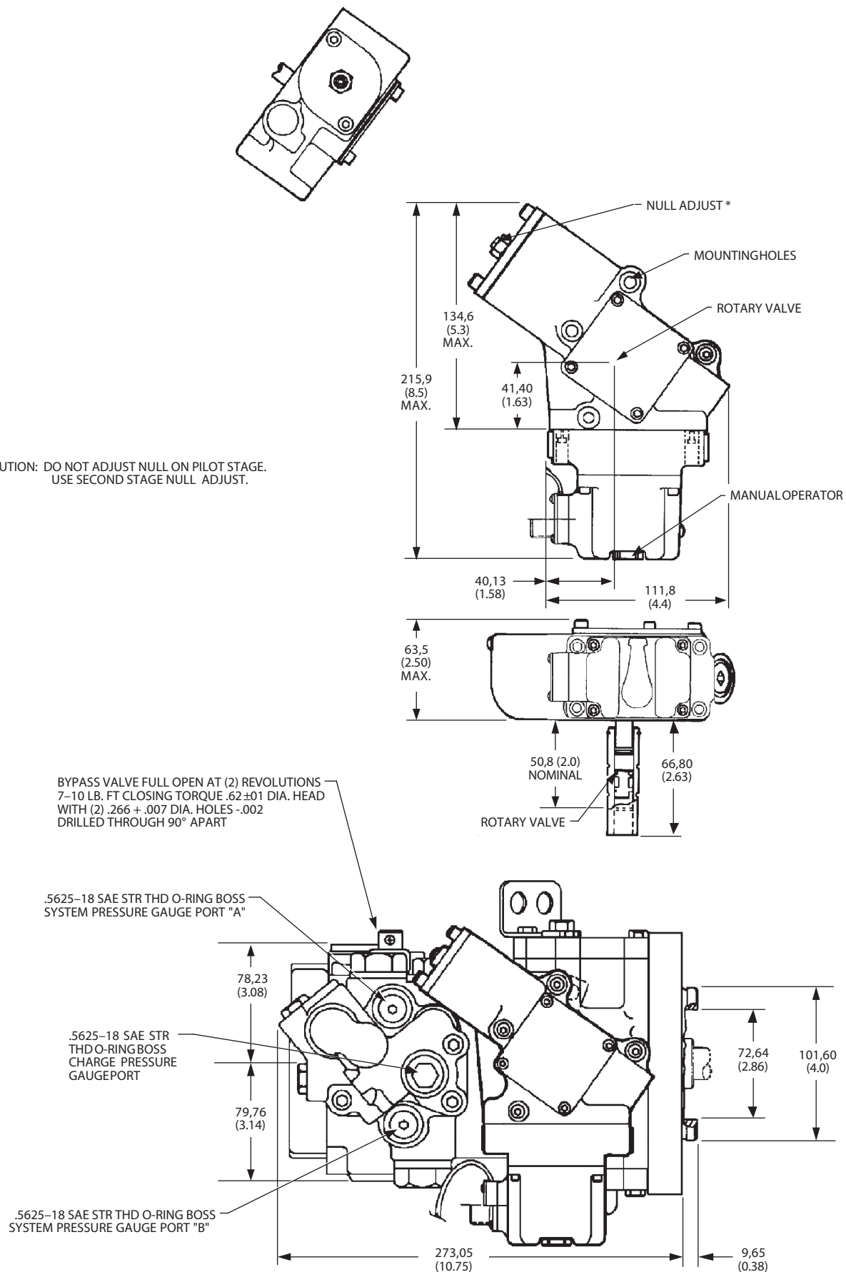
Dimensions of the MCV105C EDC in millimeters (inches).
