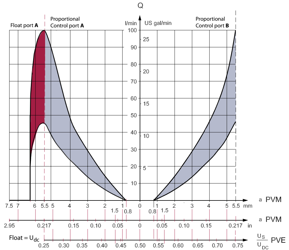
PVE characteristic – Float A
