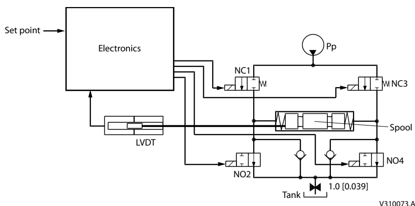
Pilot oil diagram
