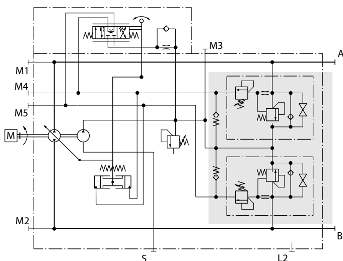
Multifunction valve, pressure limiter, pressure regulation, option 1
