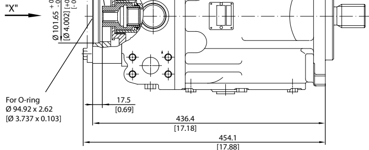
SAE C, option CD
