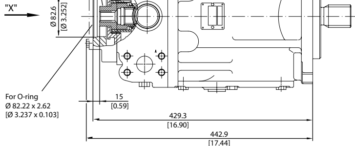
SAE B, option BC
