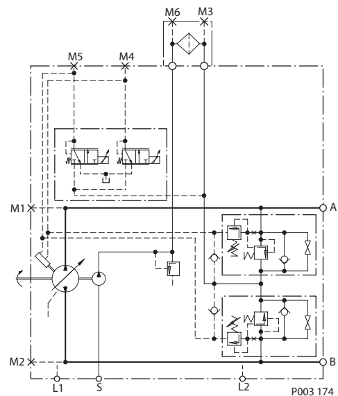
NFPE Schematic
