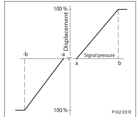
Hydraulic signal pressure range*
