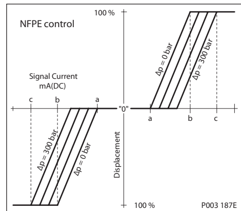
Pump Displacement vs. Input Signal
