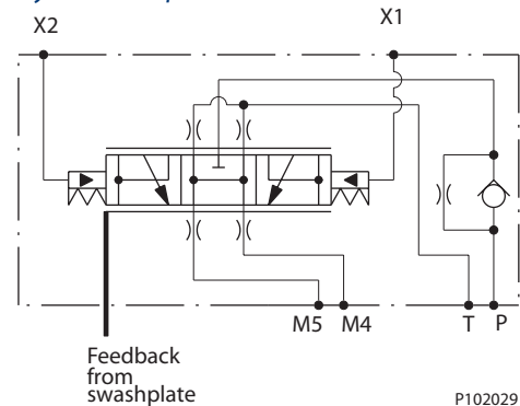
Hydraulic displacement control schematic
